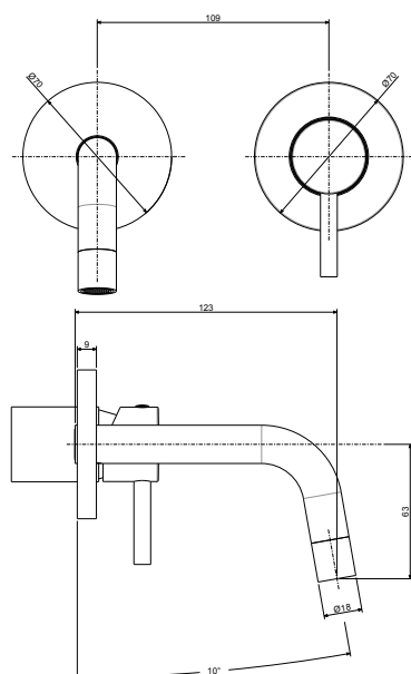
LIGBOX104RMSP70
